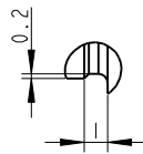
DETAIL A SCALE 12:1
