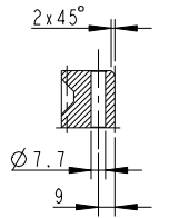
SECTION B-B
