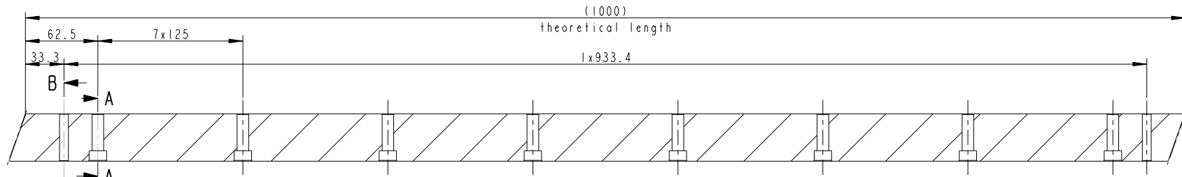
SECTION C-C
